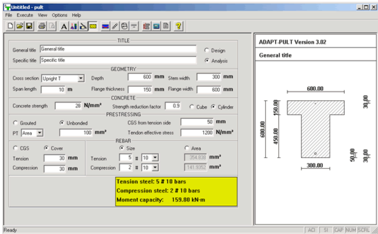
Image 1. ADAPT-PULT Screen in analysis mode
